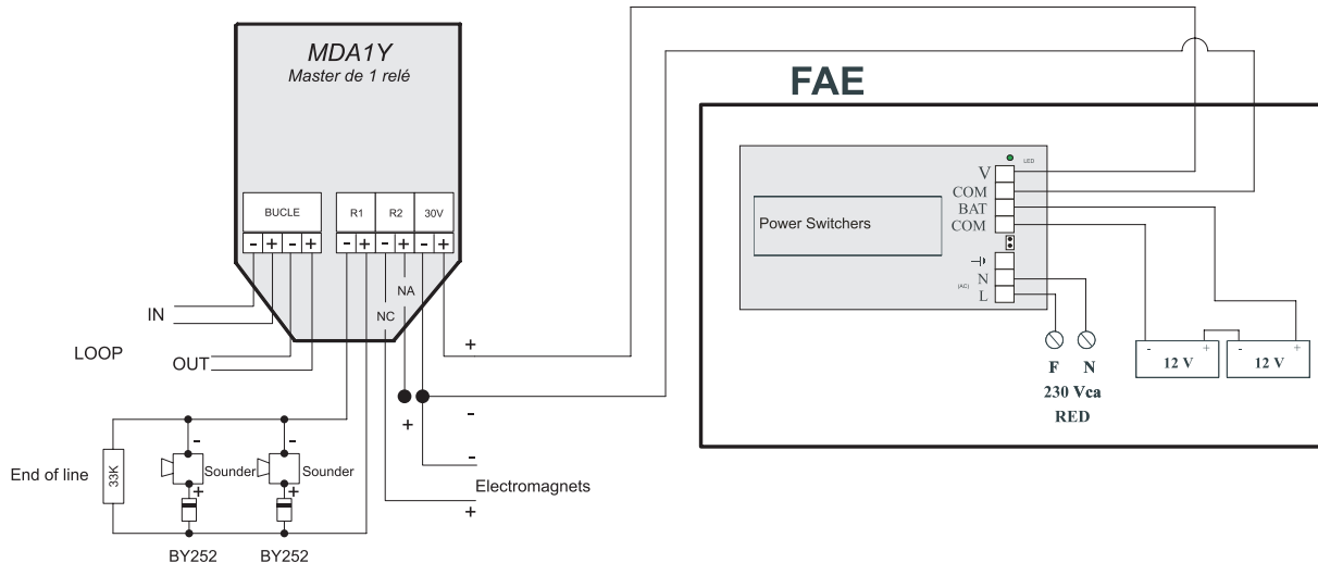
Wiring diagram F AE03/05 with relays module
