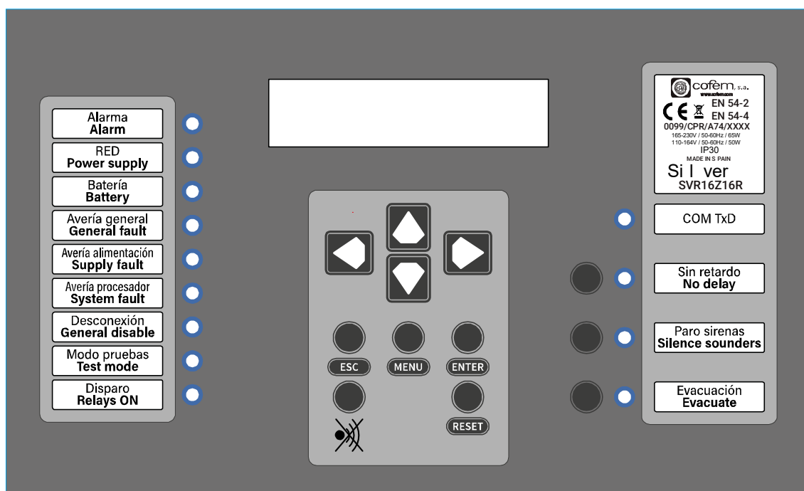
Figura 7: Panel de control de la central Silver
