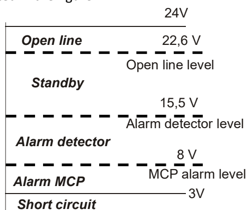
Figure 8: Zone Voltage thresholds.
